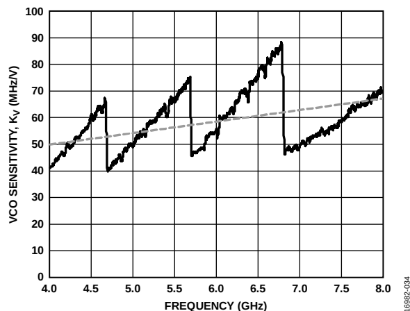
Figure 40. VCO Sensitivity, K_V vs. Frequency VCC\_VCO = 3.3\text{ V}
