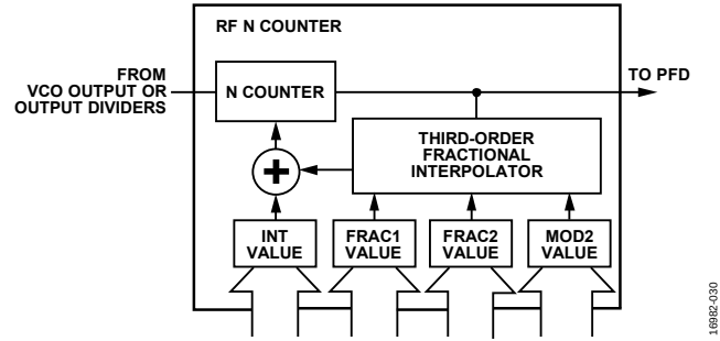
Figure 36. RF N Divider
