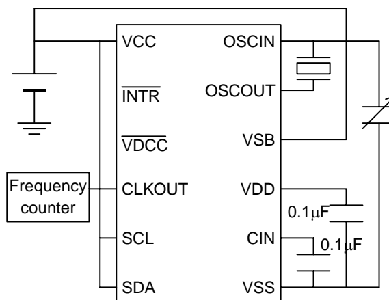
Test circuit
