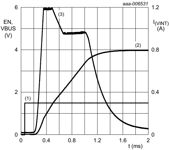
Fig 17. Typical enable time and in-rush current
