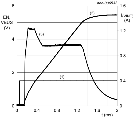
Fig 18. Typical enable time and in-rush current
