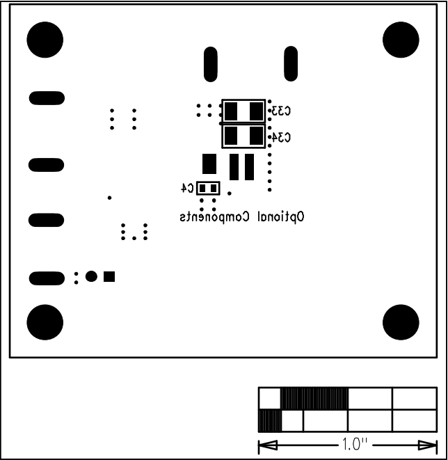
Figure 2. MAXM17516 Component Placement Guide—Solder Side
