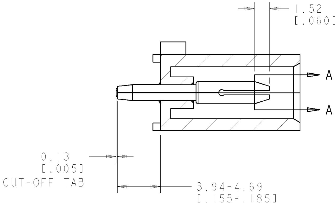
SECTION B-B
