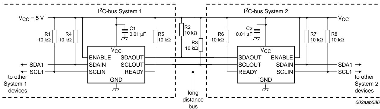
Fig 9. Repeater and bus extender application using the PCA9510A
