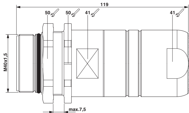
Dimensioned drawing
