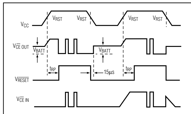
Figure 6. Chip-Enable Timing
