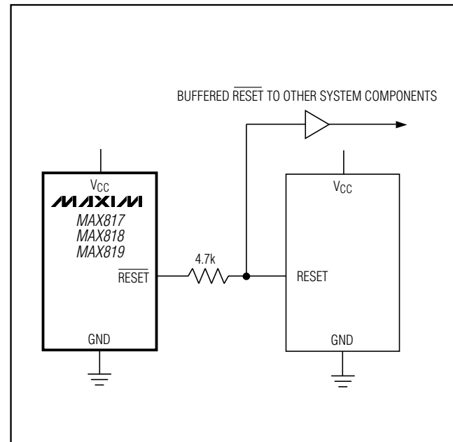
Figure 14. Interfacing to µPs with Bidirectional Reset I/O
