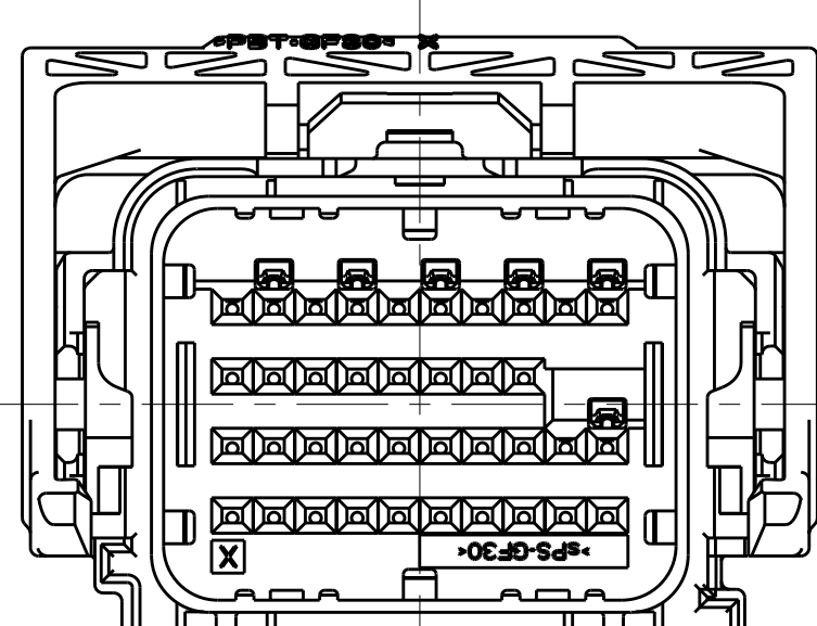
OPTION "M"
