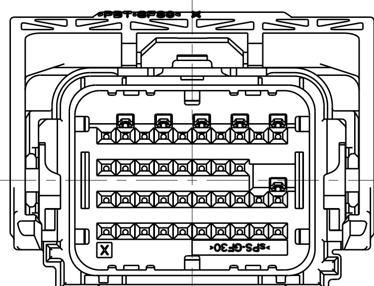
OPTION "K"
