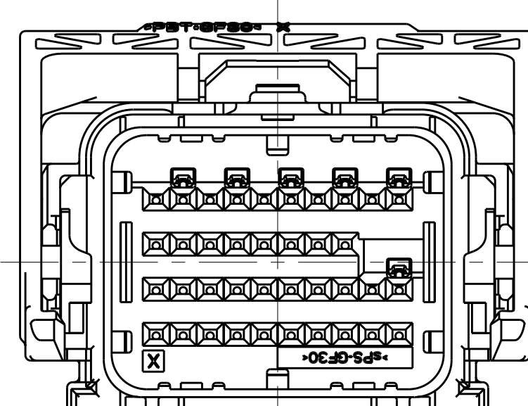
OPTION "L"
