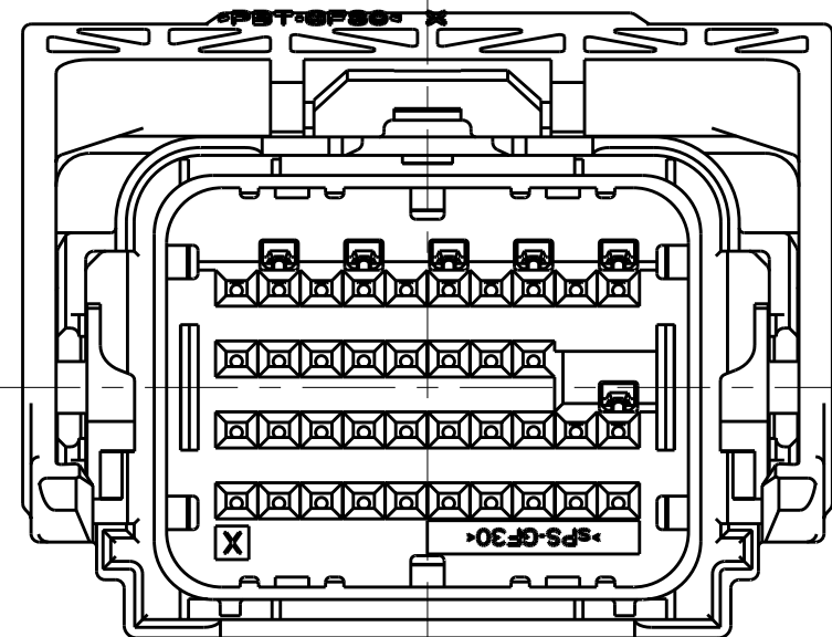
OPTION "H"
