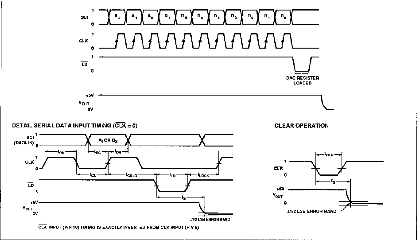
FIGURE 1: Timing Diagrams
