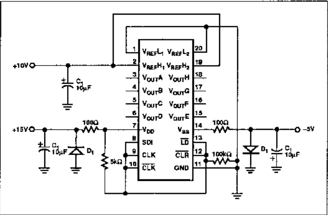
BURN-IN CIRCUIT
