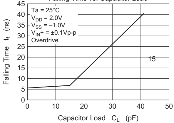
Figure 3-13 HA1631S03 Falling Time vs. Capacitor Load
