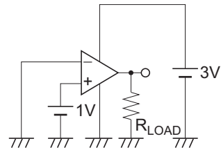
4. Output Voltage High, V_{OH}
