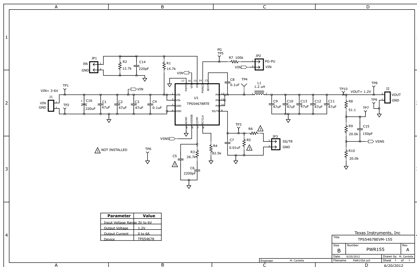
Figure 23. TPS54678EVM-155 Schematic
