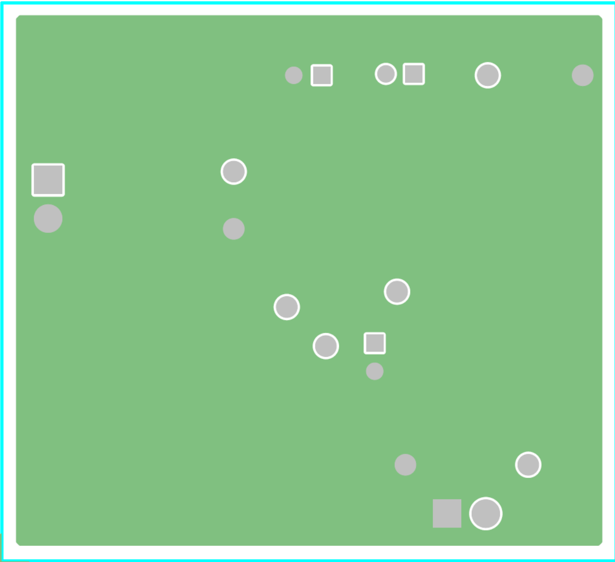
Figure 21. TPS54678EVM-155 Layout 3
