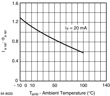
94 8020 T_{amb} - Ambient Temperature ( ^{\circ}C ) Fig. 8 - Relative Radiant Intensity/Power vs. Ambient Temperature
