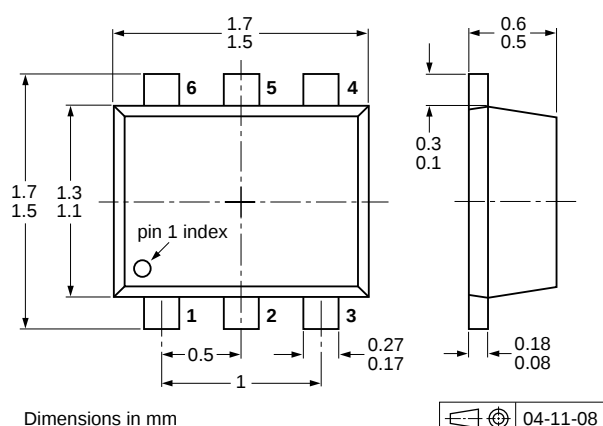
Fig 16. Package outline PEMD15 (SOT666)
