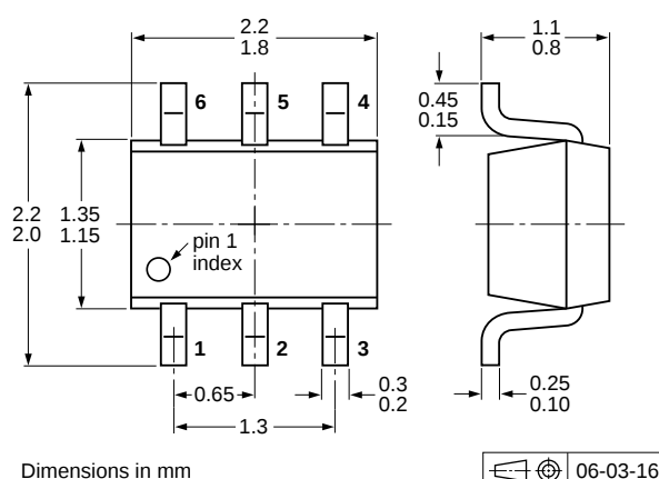
Fig 17. Package outline PUMD15 (SOT363)
