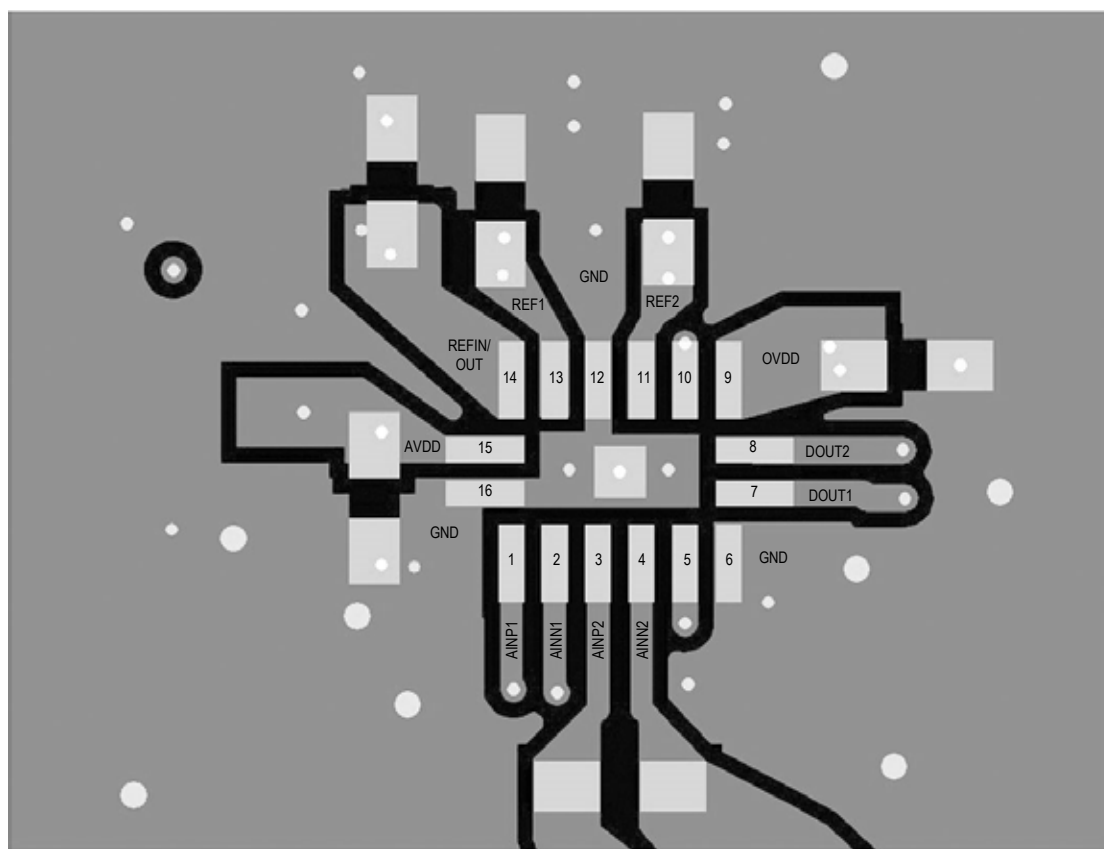
Figure 15. PCB Layout Example for MAX11192/MAX11195/MAX11198
