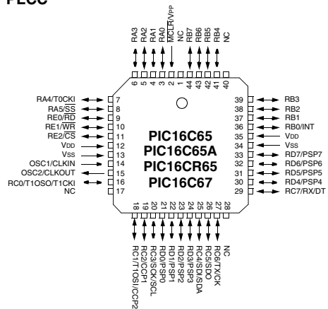
PLCC
