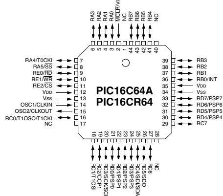
PLCC
