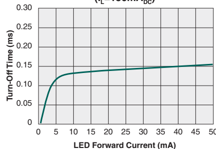
Typical Turn-Off Time vs. LED Forward Current ( I_L=130\text{mA}_{DC} )
