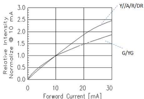
Fig 2. Relative Intensity vs. Forward Current
