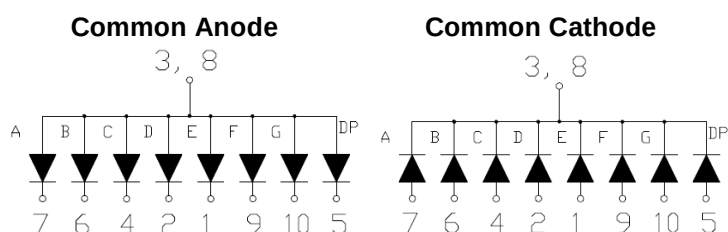
Figure 1. INND-SS40 series Internal Circuit Diagram
