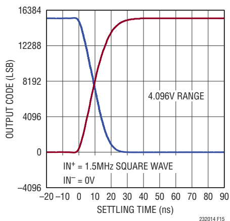
Figure 15. Transient Response of the LTC2320-14
