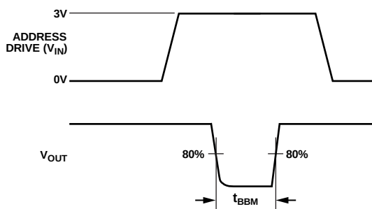
Figure 25. Break-Before-Make Delay, t_{BBM}
