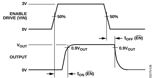
Figure 26. Enable Delay, t_{ON}(\overline{EN}) , t_{OFF}(\overline{EN})
