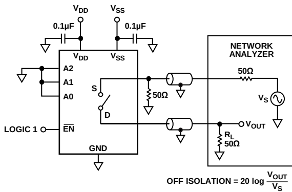
Figure 28. Off Isolation
