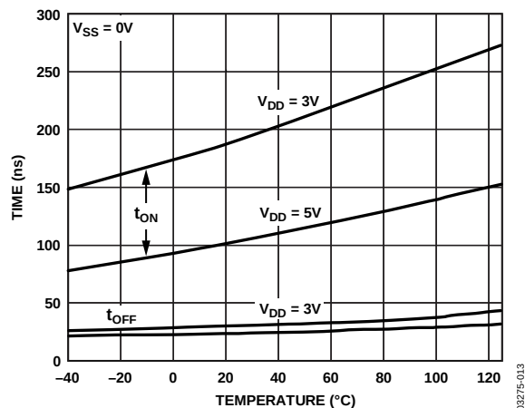
Figure 13. t_{ON}/t_{OFF} Times vs. Temperature, Single Supply
