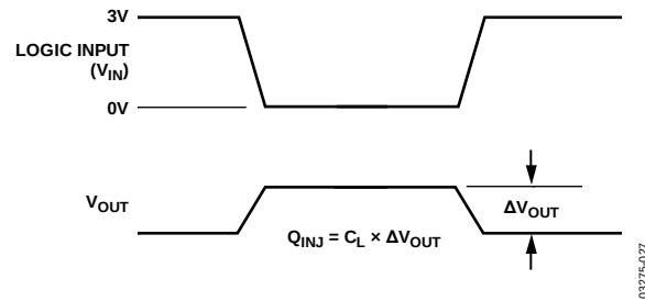
Figure 27. Charge Injection
