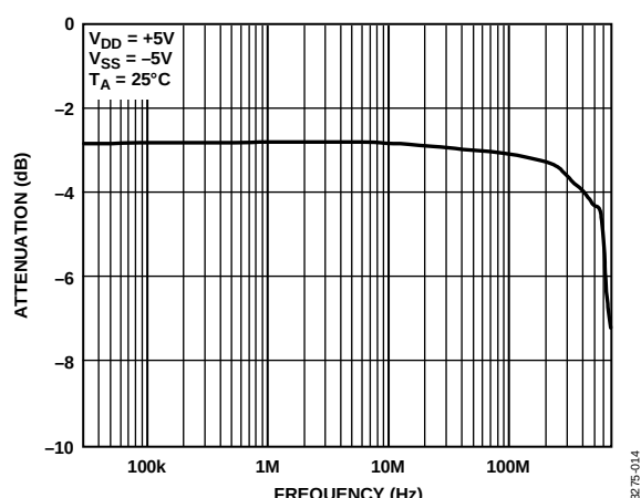
Figure 14. On Response vs. Frequency
