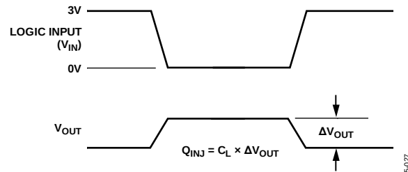
Figure 27. Charge Injection
