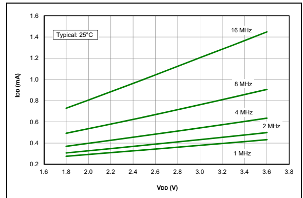
FIGURE 33-23: I_{DD} Typical, HFINTOSC Mode. PIC16LF1704/8 Only.
