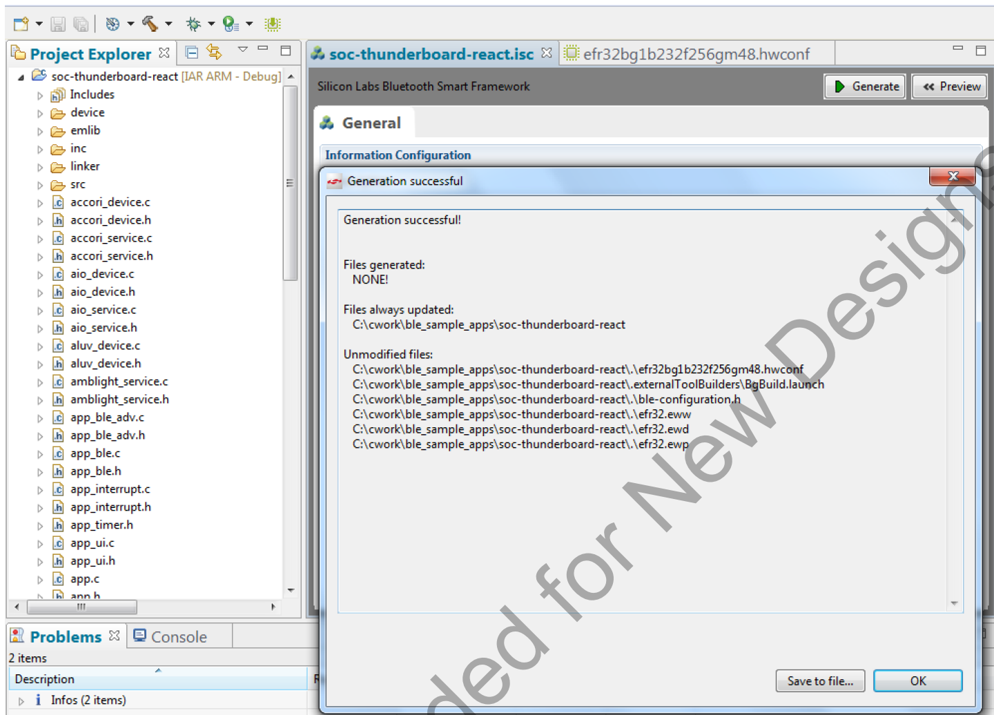
Figure 6.10. Project Generation
