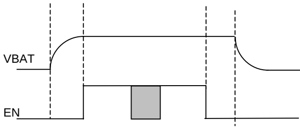
Figure 7. Power sequence
