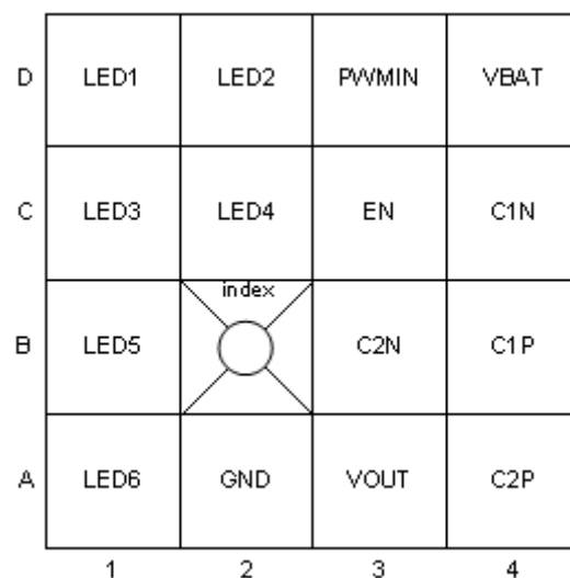
Figure 1. Pin Configuration
