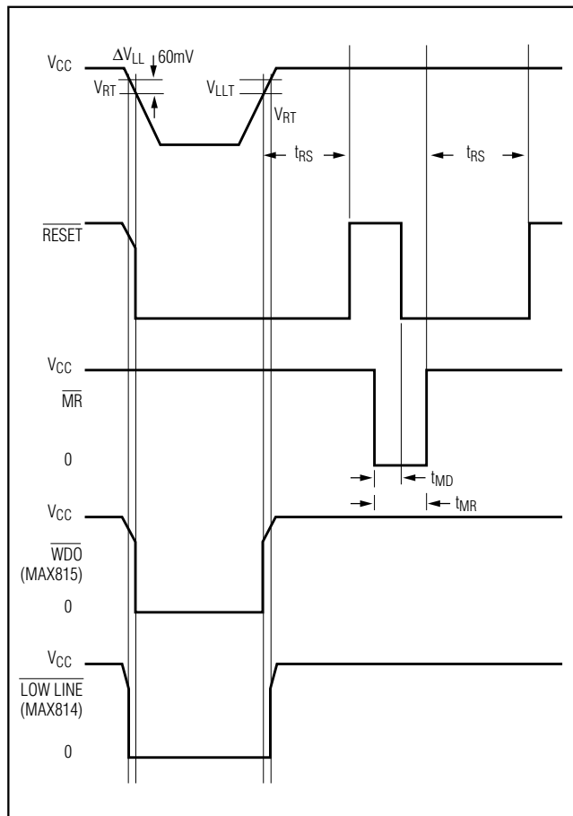
Figure 9. Timing Diagram
