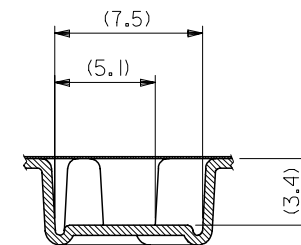
SECT:X-X (SCALE 4:1)
