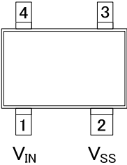
SSOT-24 (TOP VIEW)
