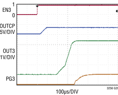
OUT3 Power-Up
