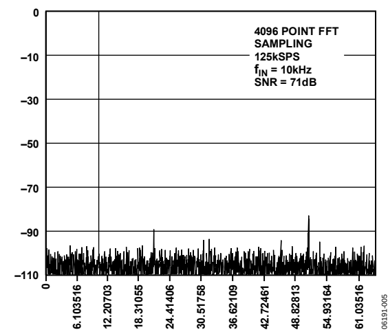
Figure 5. Dynamic Performance
