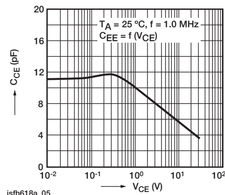
Fig. 7 - Transistor Capacitance
