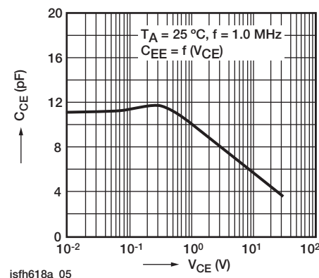
Fig. 7 - Transistor Capacitance
