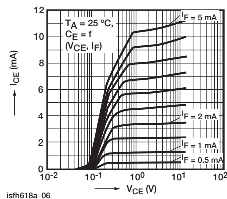
Fig. 8 - Output Characteristics
