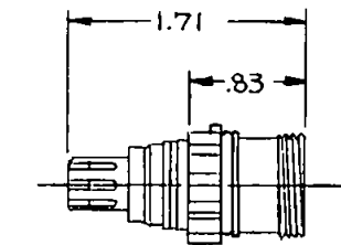
AP-107-28 PLUG, BODY ASSEMBLY
