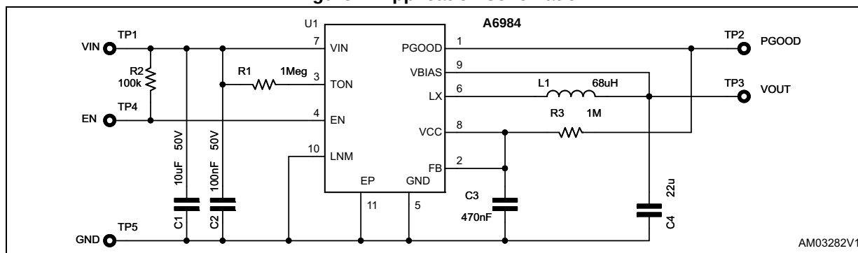
Figure 1. Application schematic
