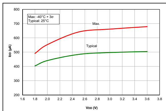
FIGURE 33-49: I_{PO} , Comparator, NP Mode ( CxSP = 1 ), PIC16LF1705/9 Only.
