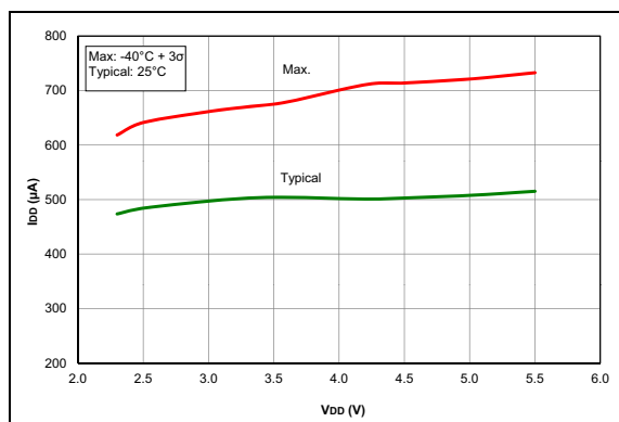
FIGURE 33-50: I_{PO} , Comparator, NP Mode ( CxSP = 1 ), PIC16F1705/9 Only.
