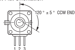
FLATTED SHAFT
