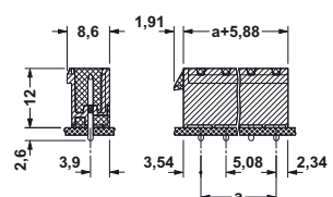
CCVA 2,5/...-GR-5,08RNP26THR
