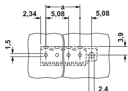
CCV 2,5/...-GFL-5,08P26THR
