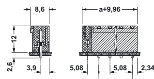
CCV 2,5/...-GFR-5,08P26THR
