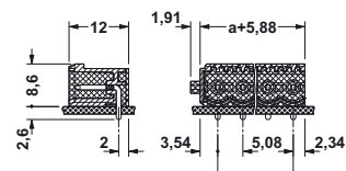
CCA 2,5/...-GL-5,08RNP26THR
