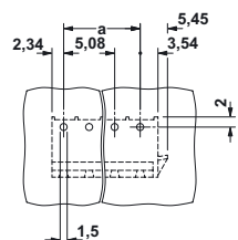
CCA 2,5/...-GR-5,08RNP26THR
