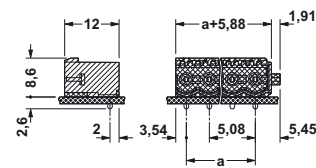
CCA 2,5/...-GR-5,08RNP26THR
