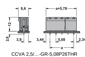
CCVA 2,5/...-GR-5,08P26THR
