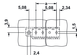
CCV 2,5/...-GFR-5,08P26THR
