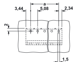
CCA 2,5/...-GL-5,08P26THR
