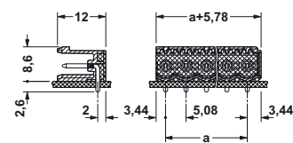
CCA 2,5/...-GR-5,08P26THR
