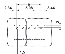
CCA 2,5/...-GR-5,08P26THR
