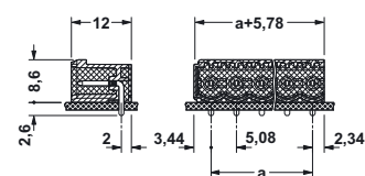
CCA 2,5/...-GL-5,08P26THR
