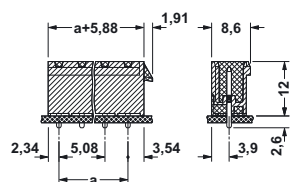
CCVA 2,5/...-GL-5,08RNP26THR
