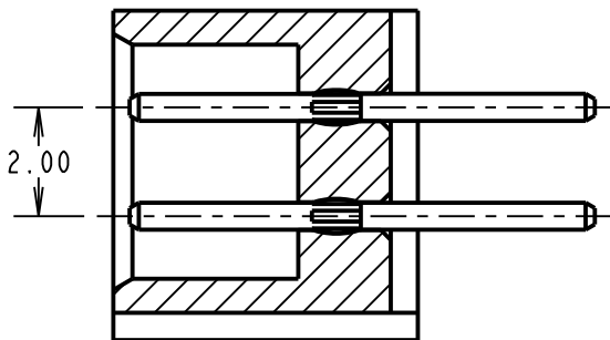
SECTION X-X
