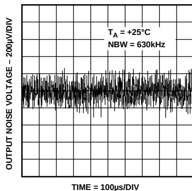
Figure 8. Broadband Noise
