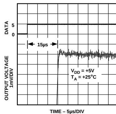
Figure 13. Output Voltage Rise Time Detail
