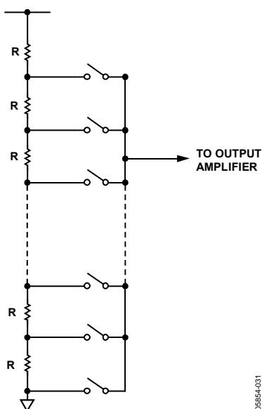
Figure 23. Resistor String
