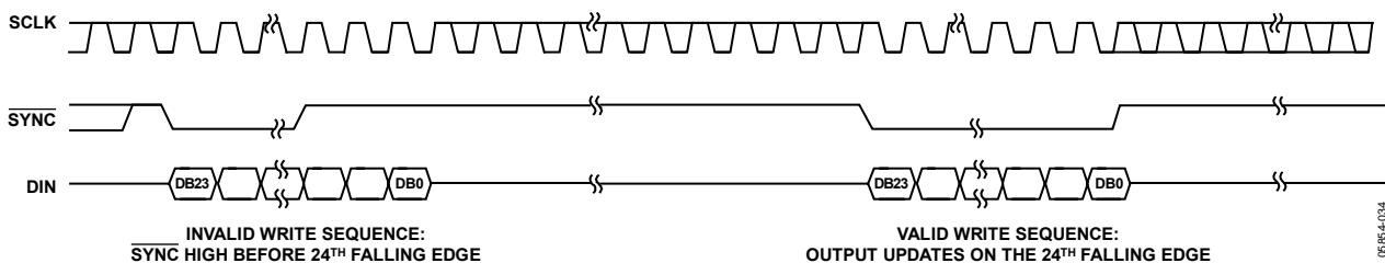
Figure 26. \overline{\text{SYNC}} Interrupt Facility
