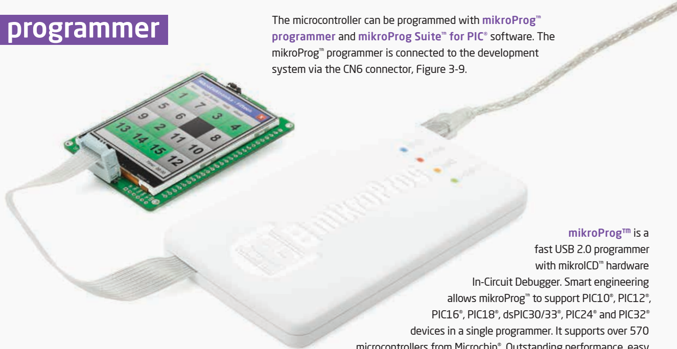
Figure 3-9: Connecting mikroProg™ to mikromedia™
