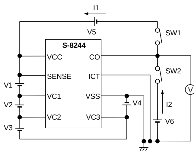
Test Circuit 4
