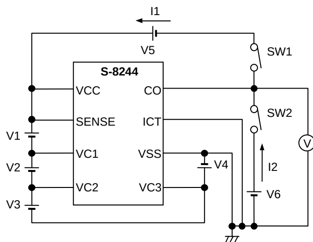
Test Circuit 4
