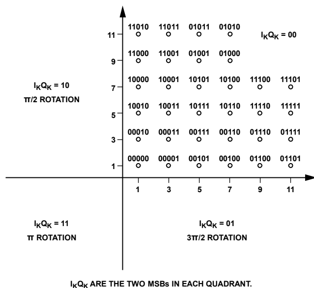
Figure 124. DVB-C 128-QAM Constellation
