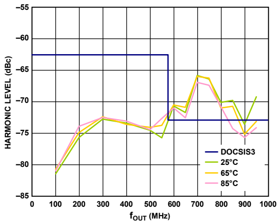
Figure 21. Second-Order Harmonic Performance vs. f_{OUT} over Temperature, 1-Channel QAM, f_{DAC} = 2.3 GHz, Full-Scale Current = 20 mA, Sum Scale = 48 (DOCSIS SPEC Is -73 dBc; Harmonic Exception Is -63 dBc)
