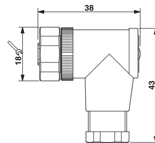
Dimensioned drawing
